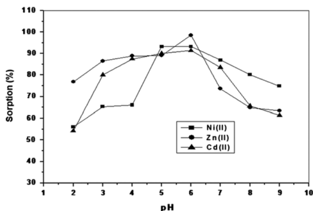
Fig. 3. Effect of pH on the extraction of Ni(II), Zn(II), and Cd(II) by 2-AT-PUF sorbent (20 mL sample, concentration of each metal ion of 1.0 \text{ mg mL}^{-1} , and 100 mg sorbent).
