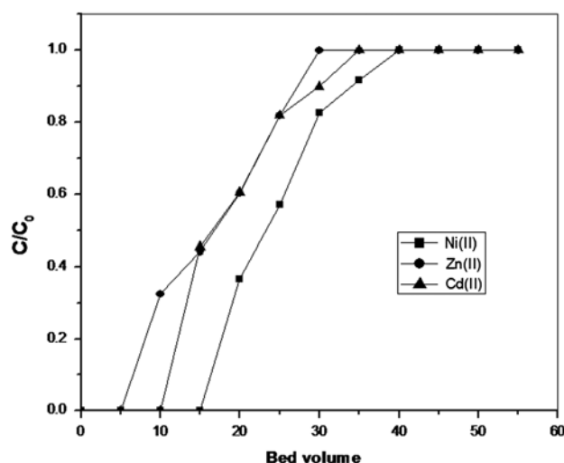
Fig. 7. Breakthrough capacity curves for Ni(II), Zn(II), and Cd(II) with 2-AT-PUF packed column at sample flow rate 3.0 mL min -1 , concentration 5.0 \mu\text{g mL}^{-1} , and pH 6.0.
