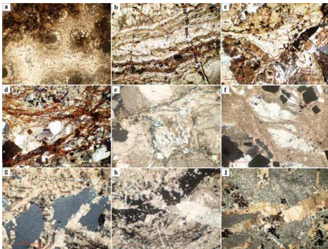
Figure 5. Photomicrographs in transmitted light: a — dolomitic spherulites with oxidized sulphide lamella and quartz in cores; b — Colloform texture formed by bands of carbonates, clay minerals and iron oxides; c — dolomite rhombs with colloform bands; d — veins of hydrothermal solution going between quartz and carbonates; e — reaction rim of hydrothermal solution with calcite in basalt; f — dissolution of quartz by carbonate solution; g — carbonate filling interspaces between amorphous silica; h — secondary calcite vein
