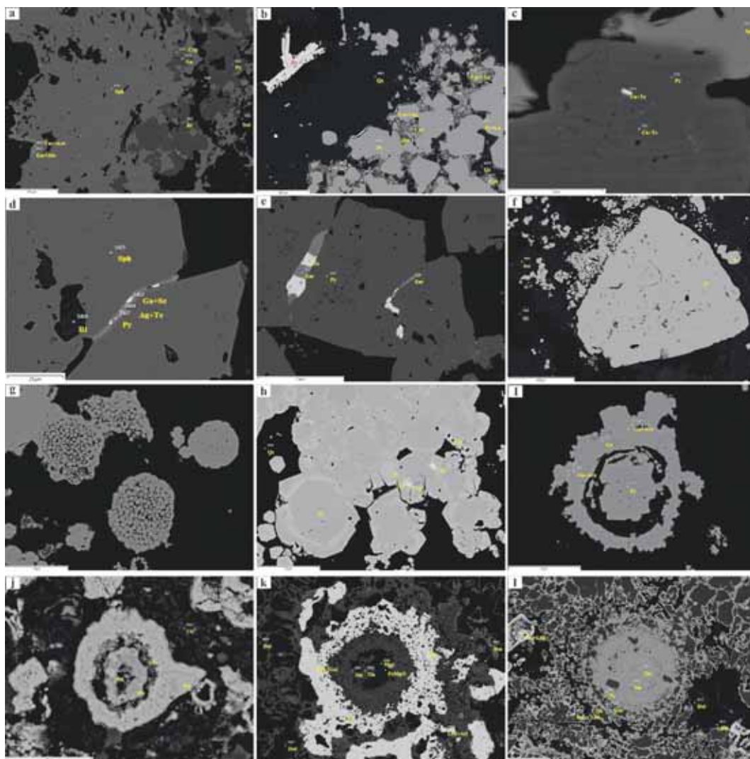
Figure 4. Backscattered electron micrographs of mineral associations and textures: a — Sphalerite porphyroblast in dolomite hosting inclusion of rutile, pyrite, chalcopyrite, and galena, and outer coating of acanthite (Ag 2 S), stibnite (Sb 2 S 3 ) and enargite (Cu 3 As 4 ); b — Silver coatings on well-crystallized pyrite and flake of barite; c — Fine inclusion of Te-rich cinnabar in pyrite; d — precipitation of galena, pyrite and Ag
