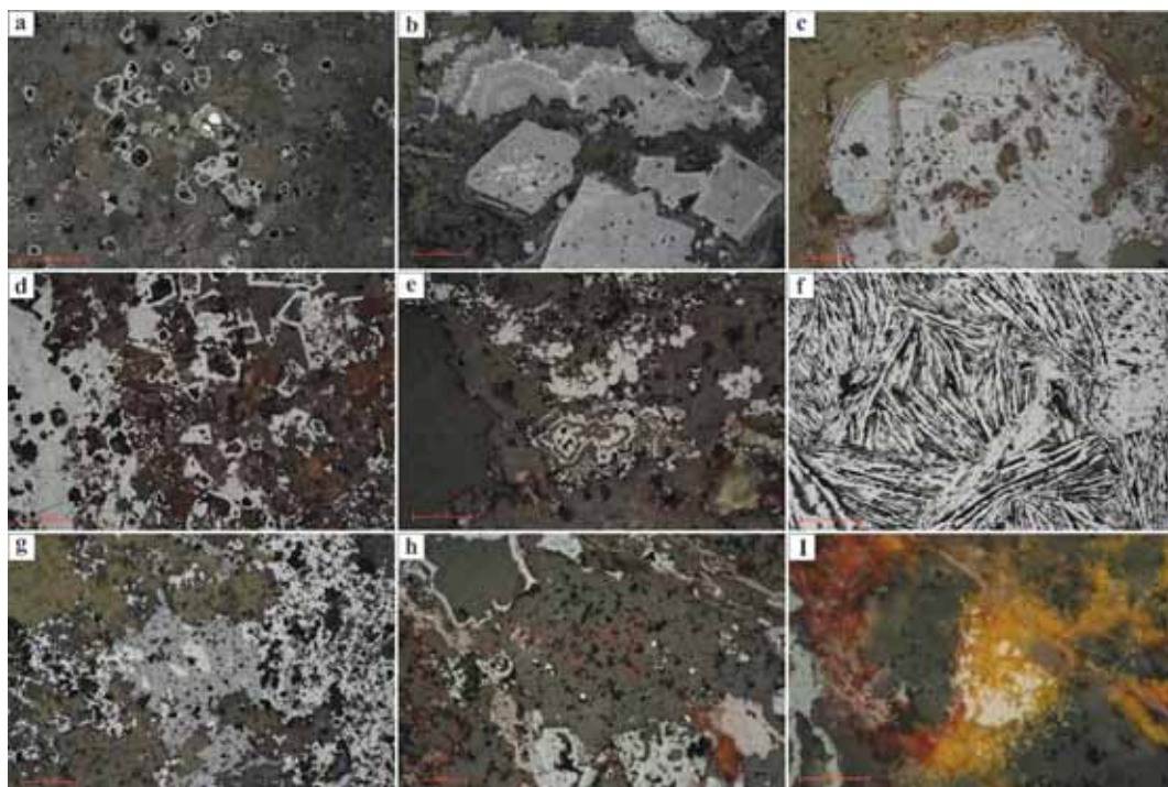
Figure 6. Photomicrographs in reflected light: a — Oxidized sulphides with relict of pyrite with a rim of hematite reserving pyrite cubic shape; b — Colloform texture formed by bands of goethite and hematite and euhedral cubes of oxidized pyrite; c — zoned iron oxides and hydroxides due to long term infiltration of fluid along the fracture of pyrites; d — intensively oxidized ore forming with outer rims of oxidized pyrite in a mixture of iron oxides, clay minerals and carbonates; e — oxidized framboidal pyrite and some of them surrounded by colloform hematite; f — specular hematite; g — intergrowth of hematite and goethite in quartz carbonate matrix; h — fine pyrite relicts in oxidized sulphides; i — pyrite mixed with hematite, limonite and goethite
