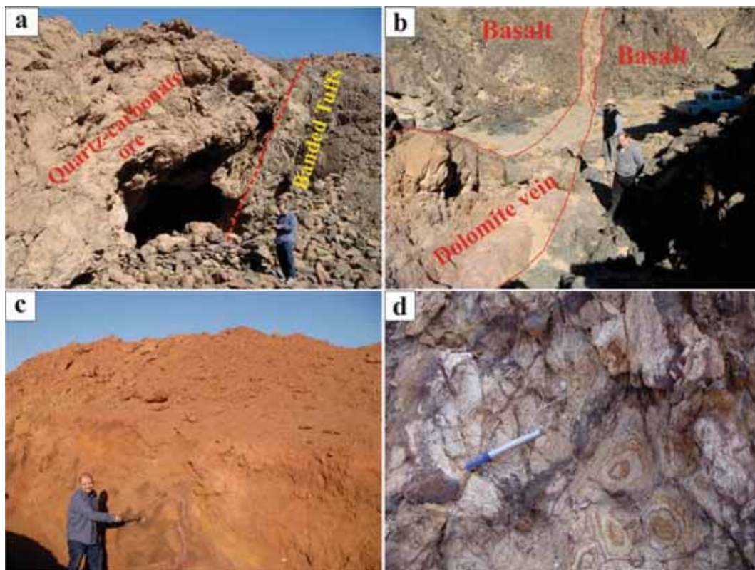
Figure 2. Different types of mineraliation in Hamama area: a — Quartz carbonate body at the contact with tuffs; b — cavity filling dolomitic veins in basalt; c — upper oxidation zone (gossan); d — foot wall alteration zones in felsic volcanics.
