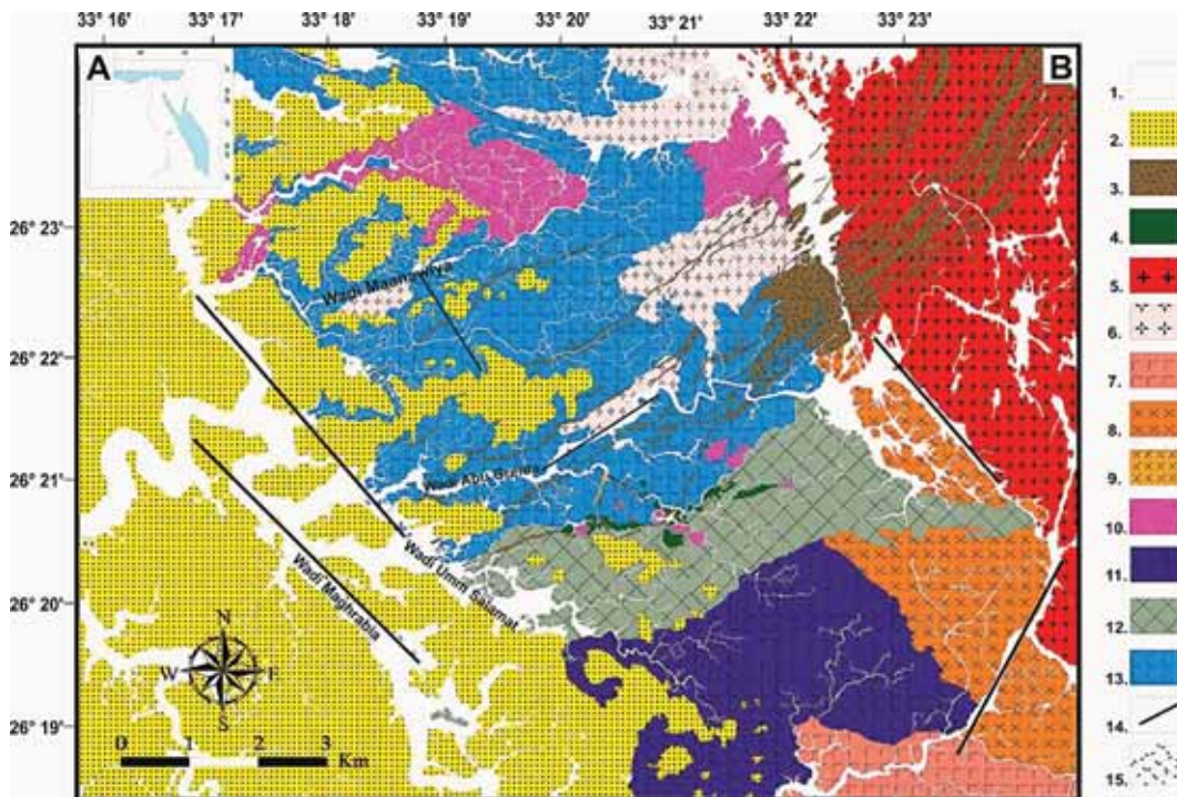
Figure 1. A — Location map, B — Geological map of the Hamama area, CED, Egypt: 1 — Wadi deposits; 2 — Sandstone; 3 — Rhyolite dykes; 4 — Quartz-carbonate ore; 5 — Monzogranite; 6 — Tonalite — trondhjemite; 7 — Gabbro; 8 — Granodirite; 9 — Quartz diorite; 10 — Acidic and intermediate volcanic; 11 —
