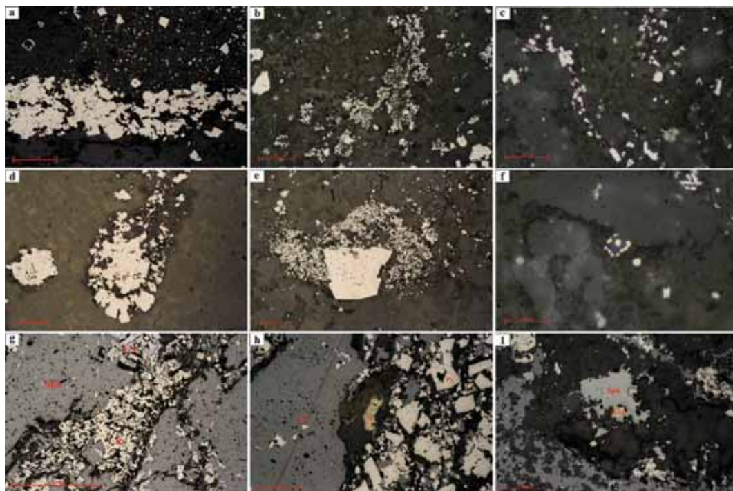
Figure 3. Photomicrographs of microfabrics in reflected light: a — Primary banding shown by alternating compositional layers of pyrite and carbonates; b — Dendriform pyrite clusters within carbonates; c — Fine
